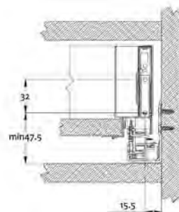
Drawer slide installation dimensions
