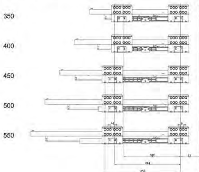
Drawer slide installation dimensions
