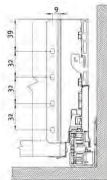
Back panel installation dimensions
