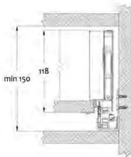
Drawer slide installation dimensions
