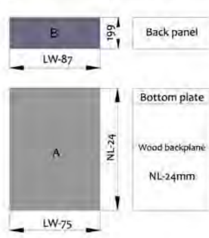
Cutting dimensions for back panel
