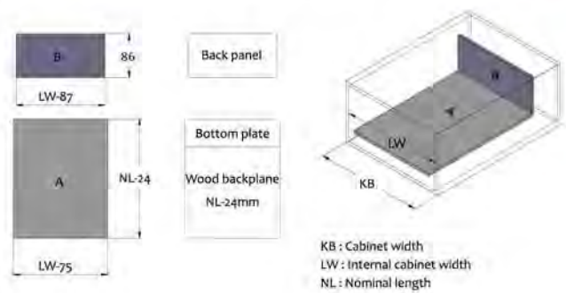
Cutting dimensions for back panel
