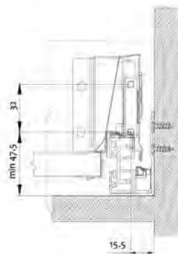
Drawer slide installation dimensions
