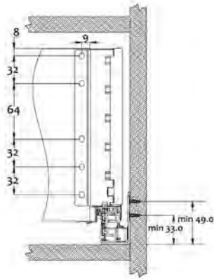
Back panel installation dimensions
