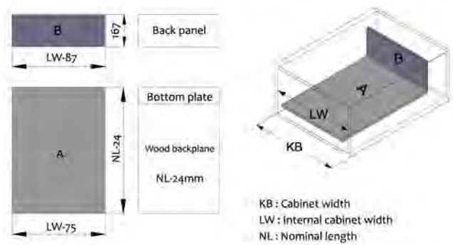
Cutting dimensions for back panel
