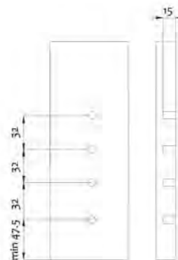
Cutting dimensions for back panel
