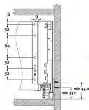
Back panel installation dimensions
