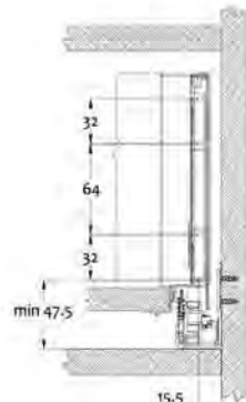
Front connector panel installation dimensions
