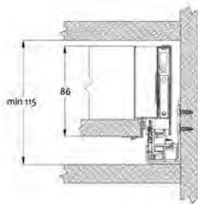
Drawer slide installation dimensions
