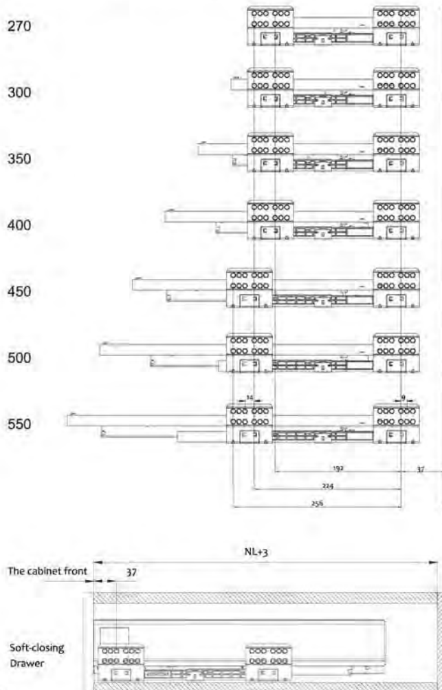
Drawer slide installation dimensions
