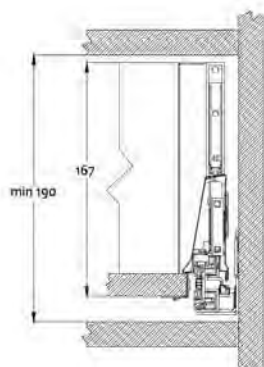
Cabinet space requirements
