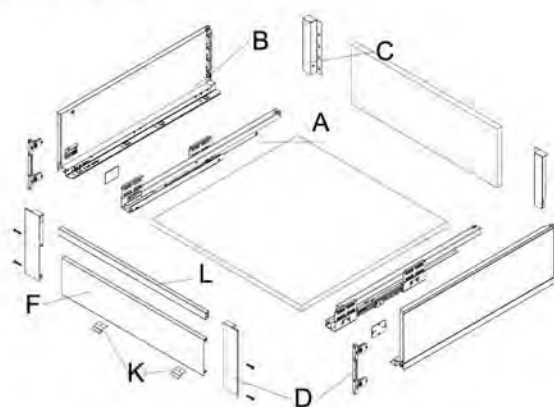
Components view
