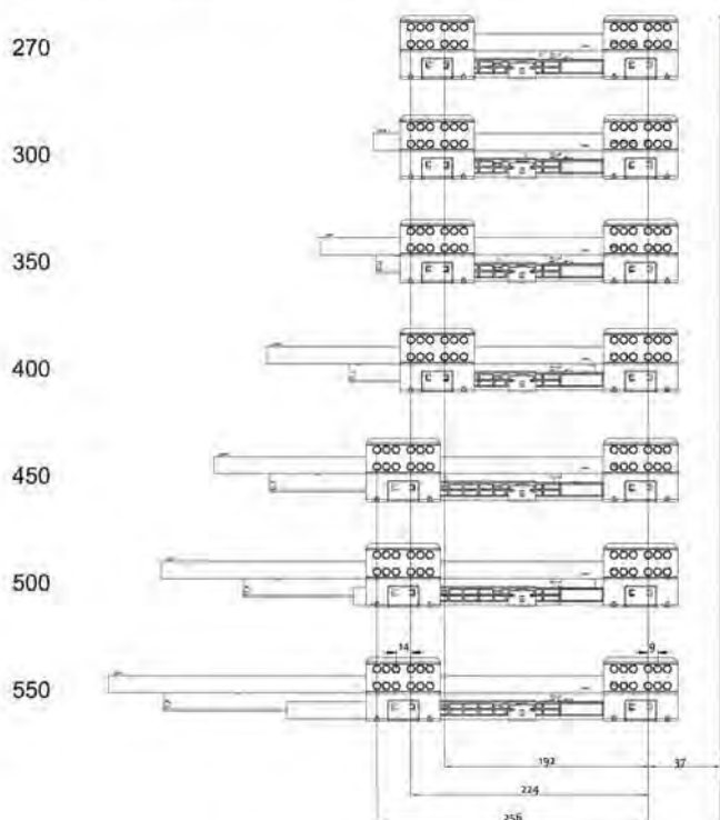
Drawer slide installation dimensions
