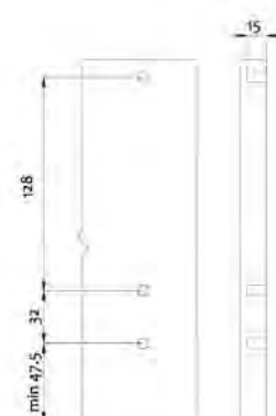
Front panel drilling dimensions
