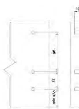
Front panel drilling dimensions
