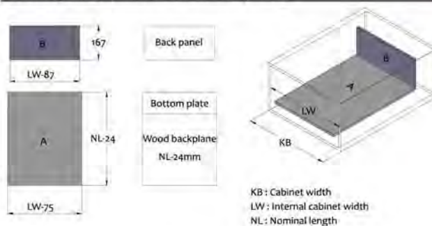
Cutting dimensions for back panel
