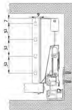
Back panel installation dimensions
