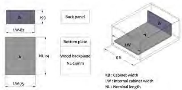
Cutting dimensions for back panel
