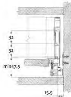
Drawer slide installation dimensions
