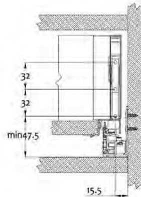
Back panel installation dimensions
