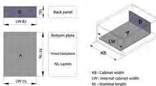
Cutting dimensions for back panel
