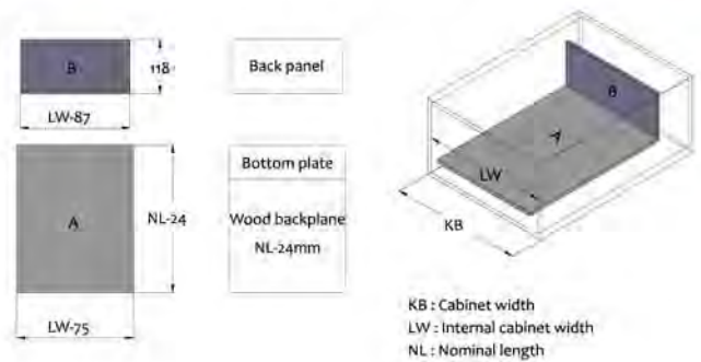
Cutting dimensions for back panel
