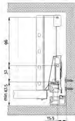
Drawer slide installation dimensions
