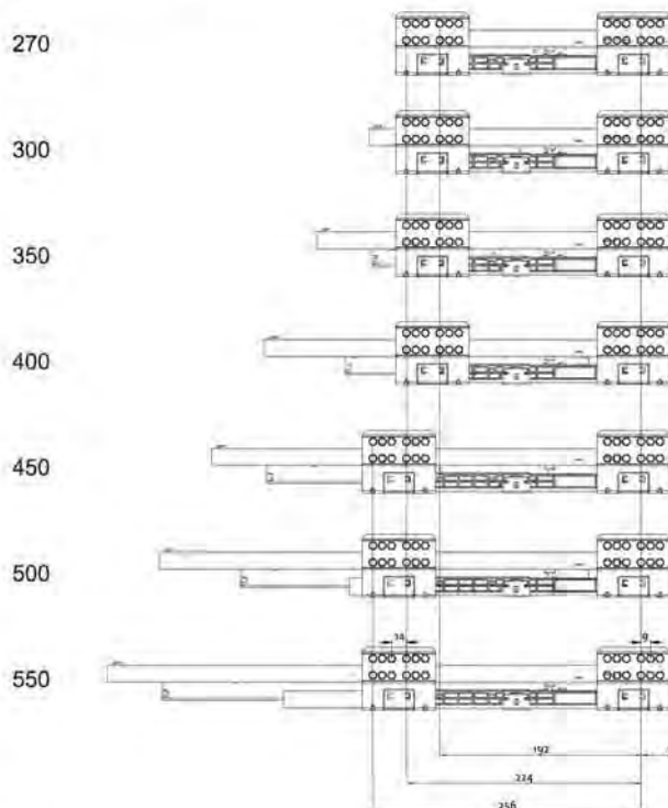
Drawer slide installation dimensions
