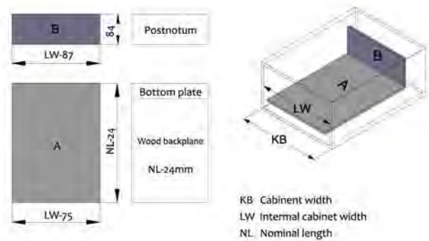
Cutting dimensions for back panel
