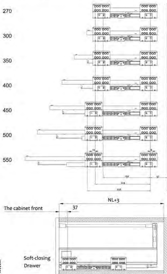
Drawer slide installation dimensions
